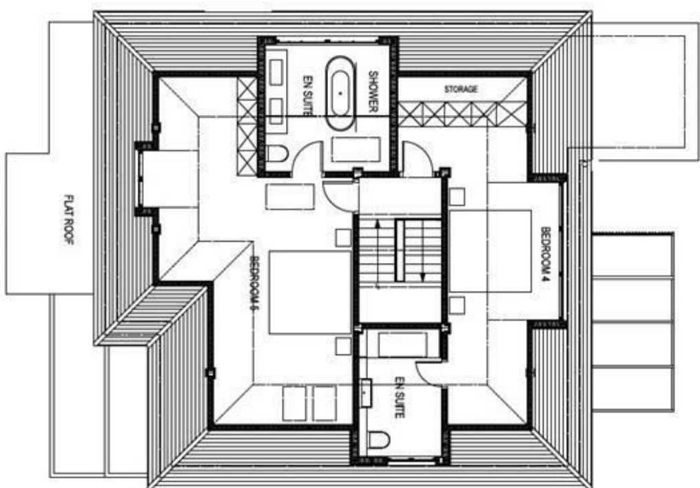
SECOND FLOOR
